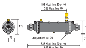
Heat Line Unequipped
