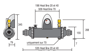
Heat Line Plus without circulating pump
