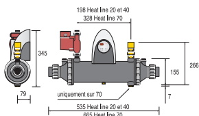
Heat Line Plus with circulating pump
