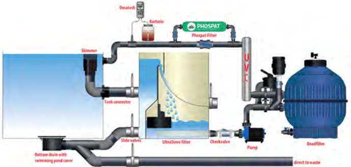
In this filter installation an AquaForte UltraSieve is used as pre-filtration.
