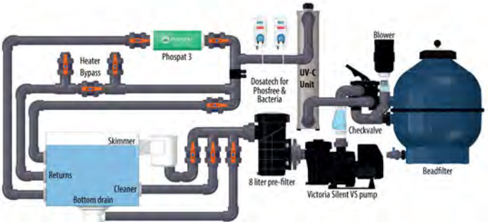
A complete plug & swim pallet was used in this above-ground filter installation.
